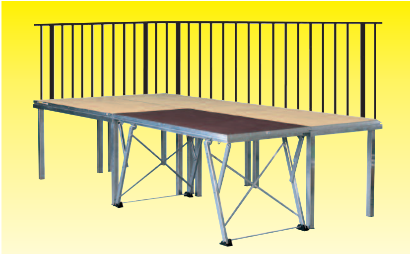
Sicherheitsgeländer DIN 4112, for Professional, Multi and Event.
